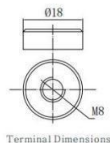
Terminal Dimensions
